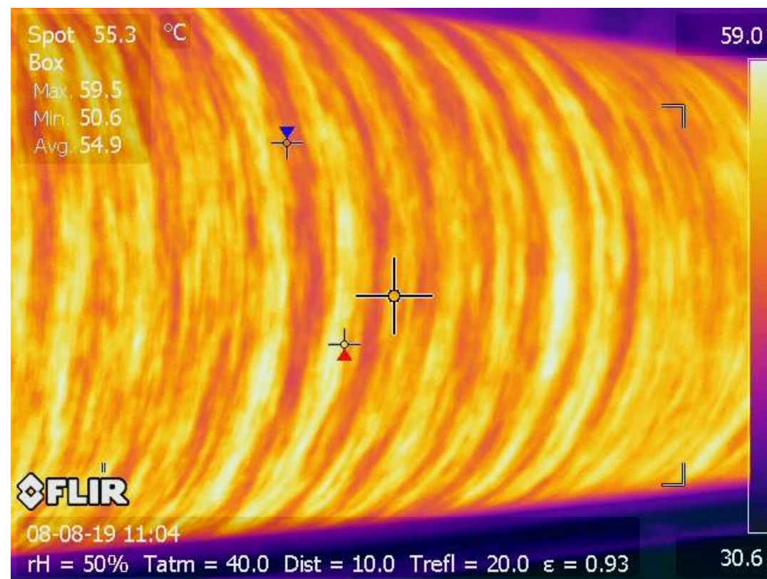
Termographic picture of tambour
